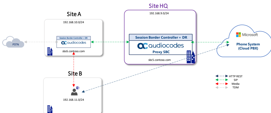
Figure 8: Always Bypass with Teams User and SBC in Different Sites
